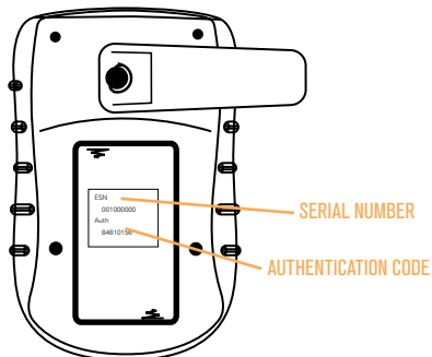
inside battery compartment
